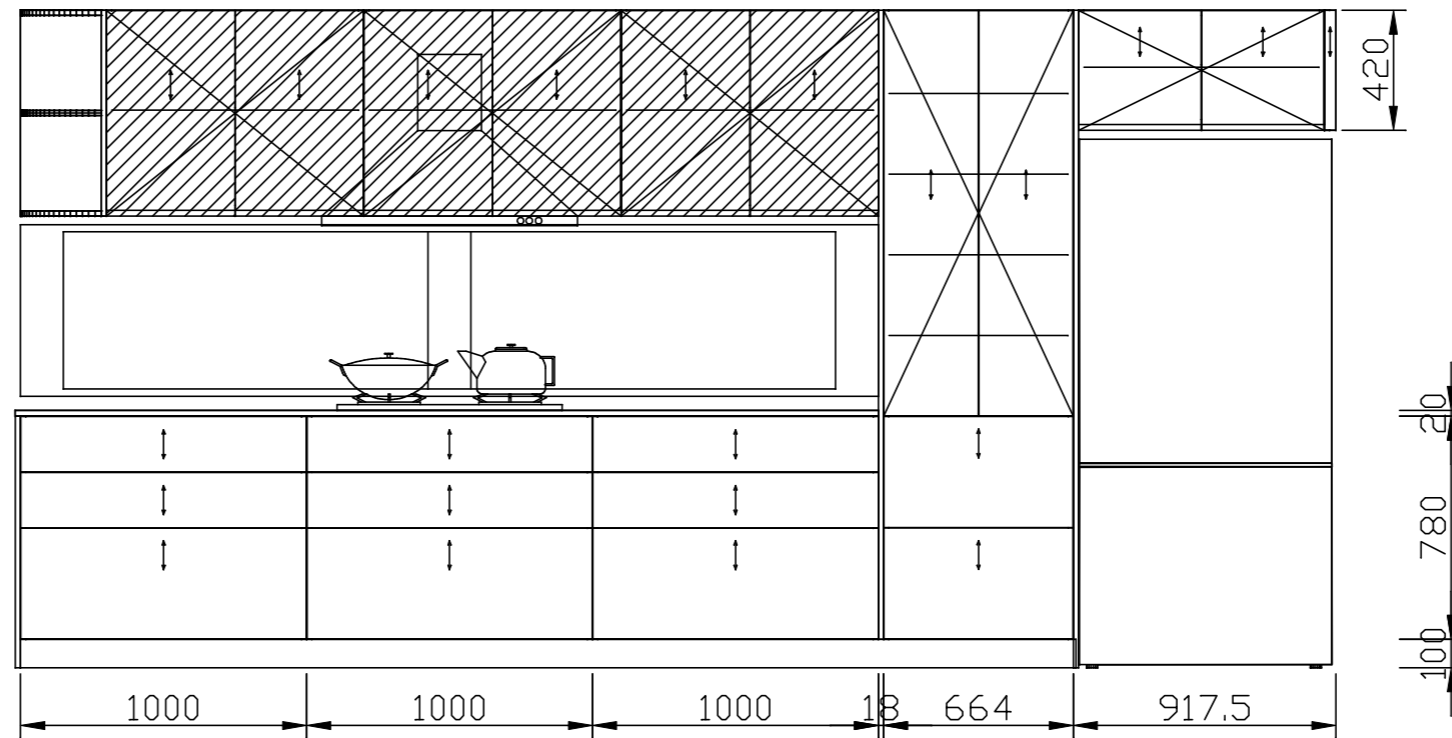
A View elevation drawing
