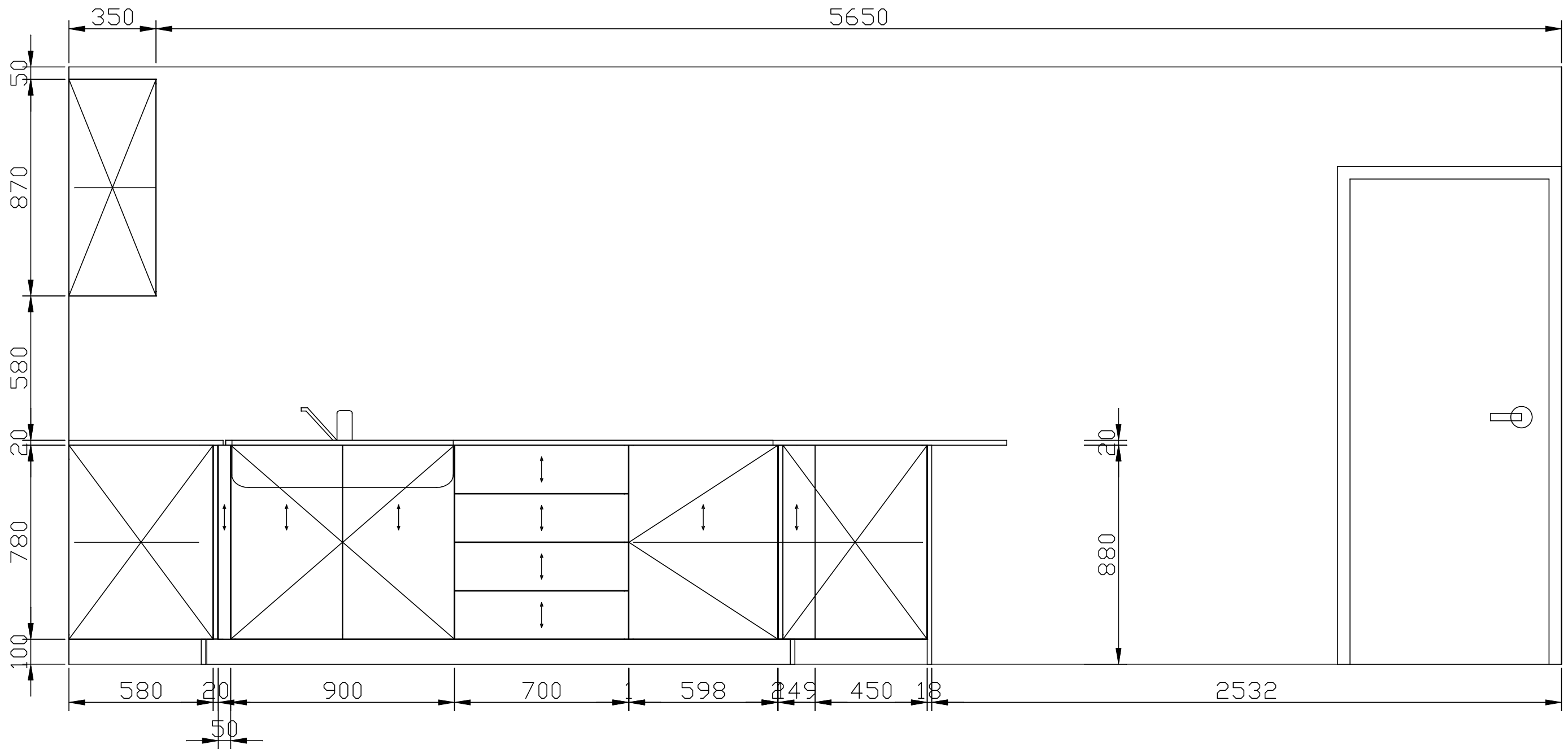
A View elevation drawing
