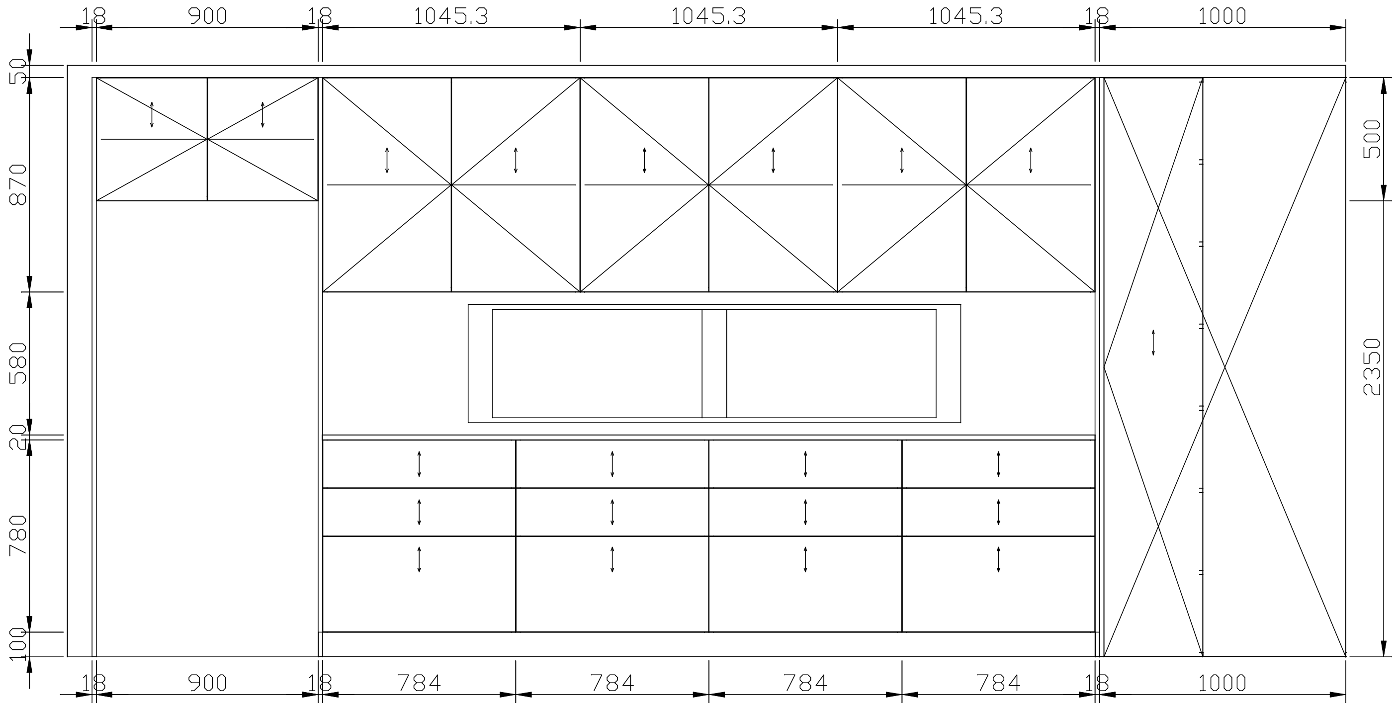
B View elevation drawing
