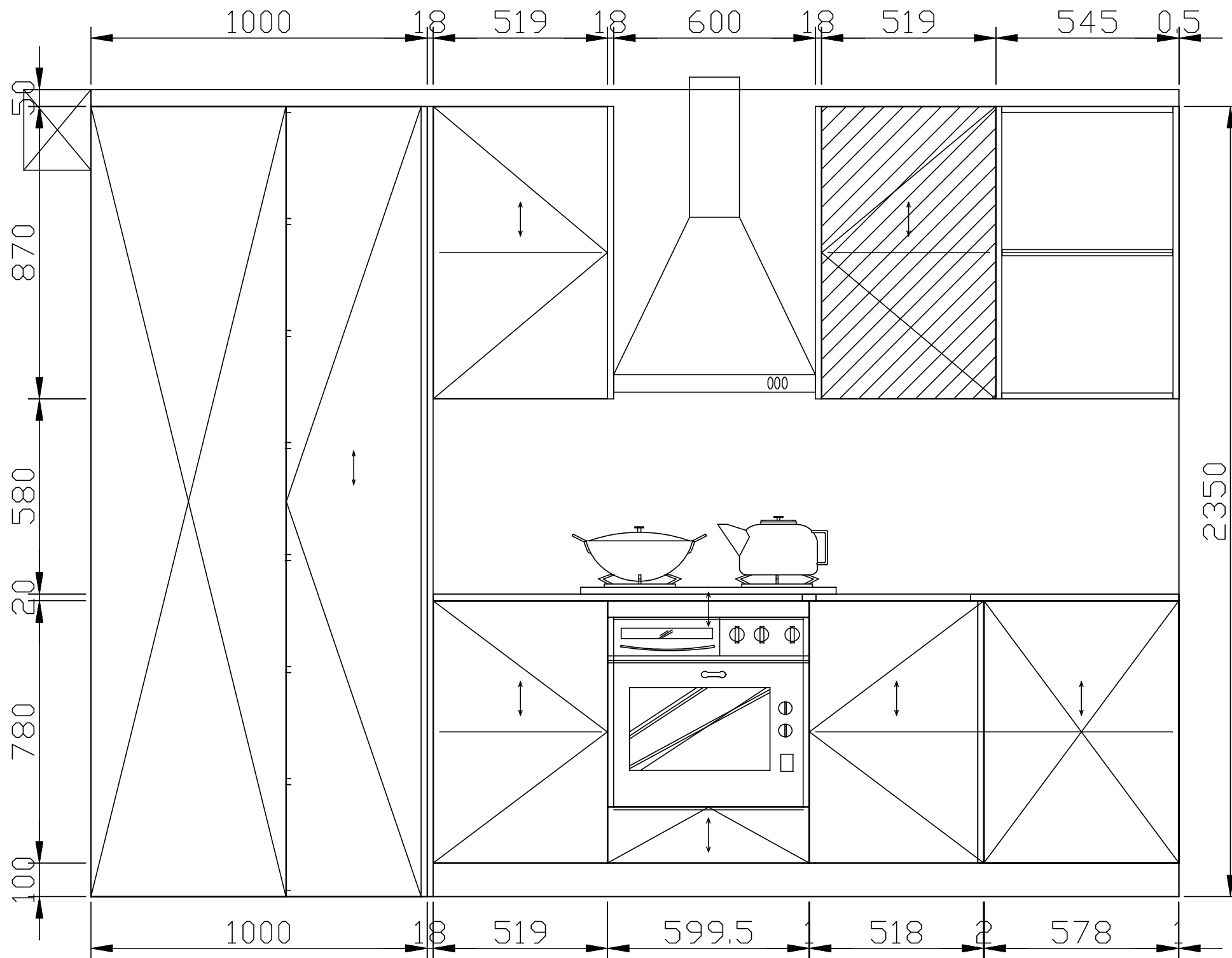
C View elevation drawing
