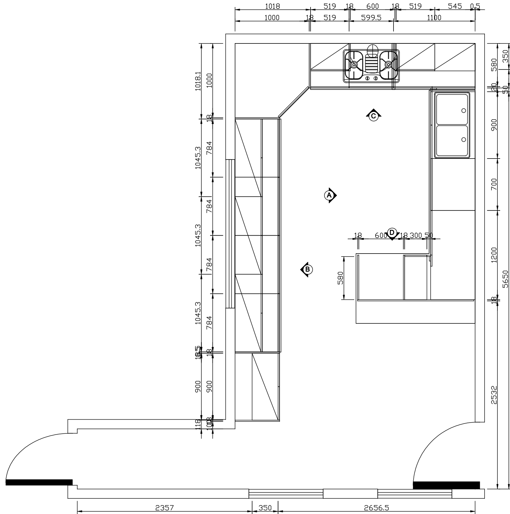
Plan drawing
