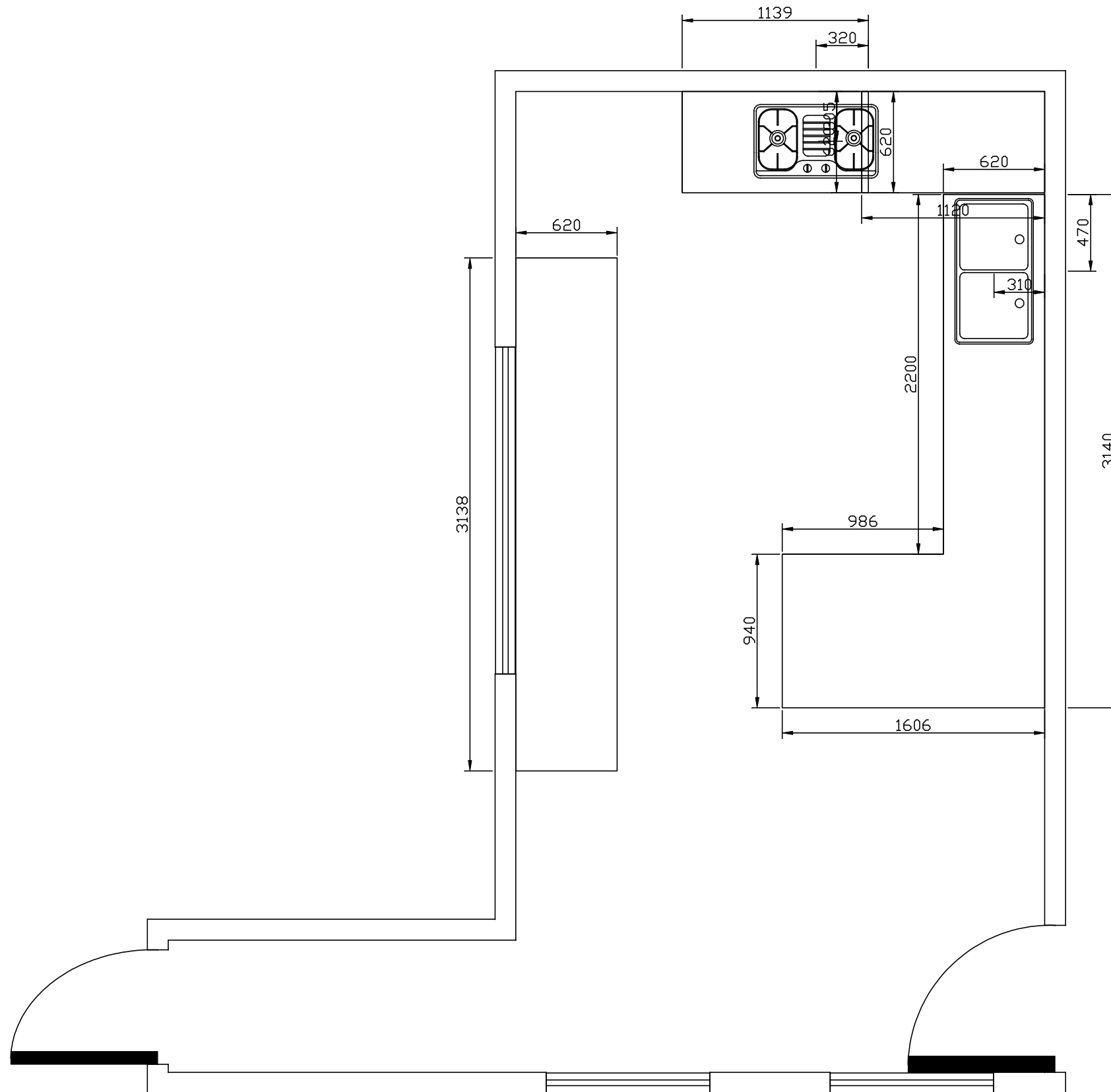
Worktop plan drawing
